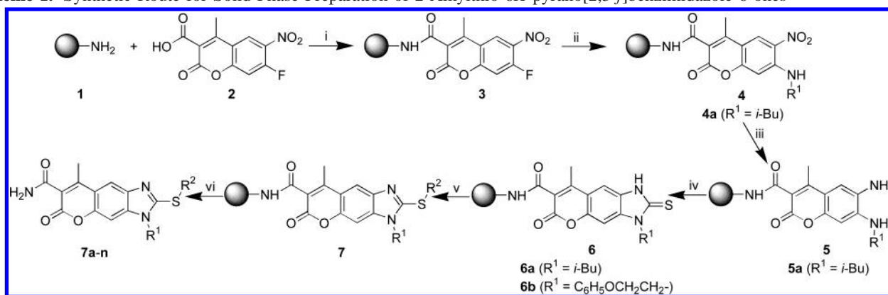
Scheme 1. Synthetic Route for Solid-Phase Preparation of 2-Alkylthio-6 H -pyrano[2,3- f ]benzimidazole-6-ones a
