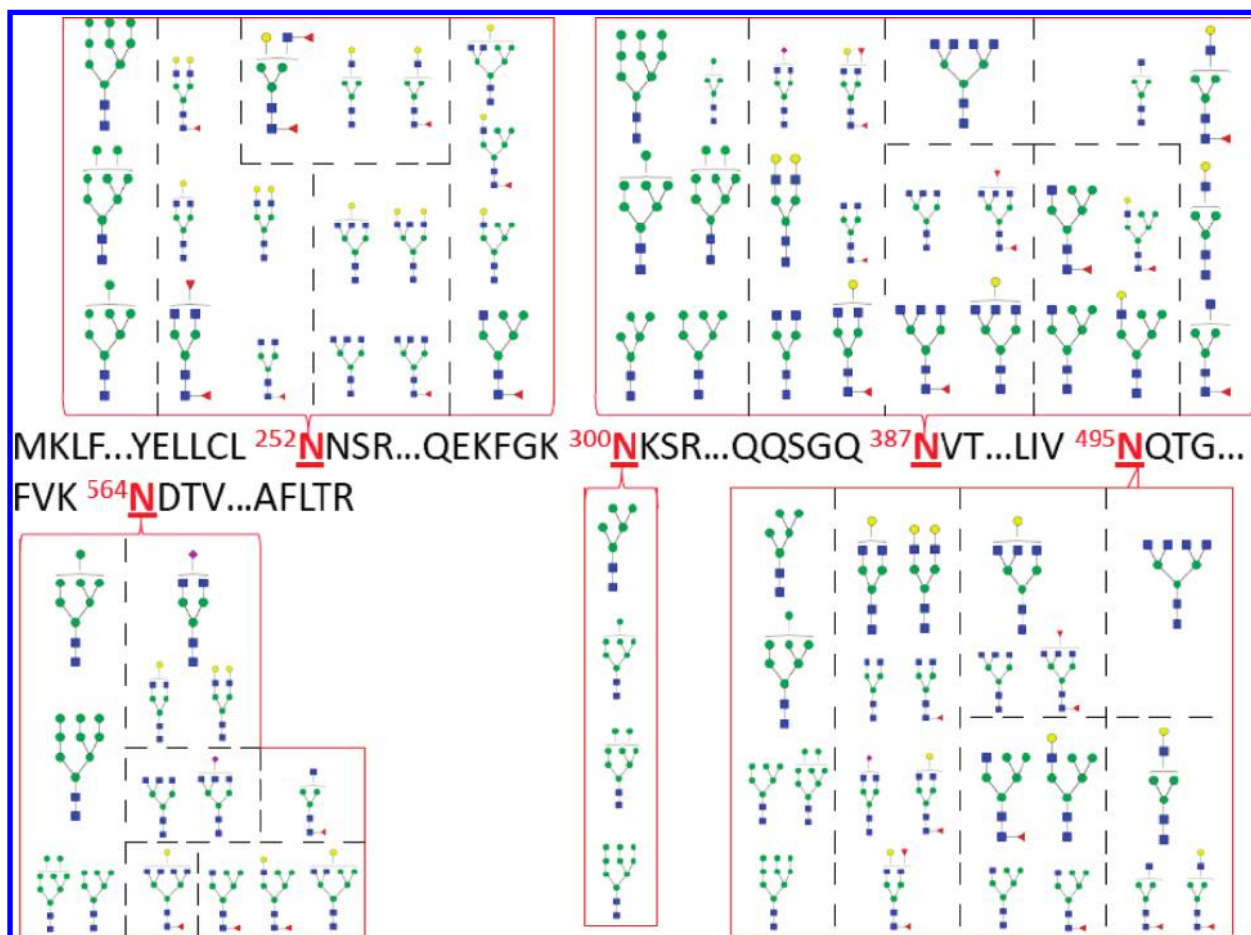
Figure 6. Glycosylation associated with each glycosite of bovine lactoferrin (b-LF). The various glycans at each site indicate glycan microheterogeneity in the occupancy of the five glycosites observed during the negative ion mode MS analysis of the b-LF glycopeptides. For each glycosite, the larger glycan structures represent corresponding glycopeptides with minimum relative intensities of 20% while the smaller glycan structures represent corresponding glycopeptides with relative intensities corresponding to less than 20%. Circles (green ● and yellow ○), squares (blue ■), and triangles (red left pointing triangle) represent hexose, GlcNAc, and fucose residues, respectively.
