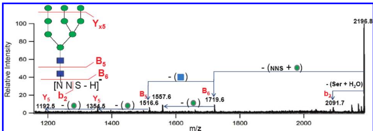
Figure 3. Negative ion mode MALDI FTICR MS/MS spectrum of precursor ion with m/z 2196.75 Da assigned as [^{252}\text{NNS} + \text{GlcNAc}_2 + \text{Man}_9 - \text{H}]^- .
