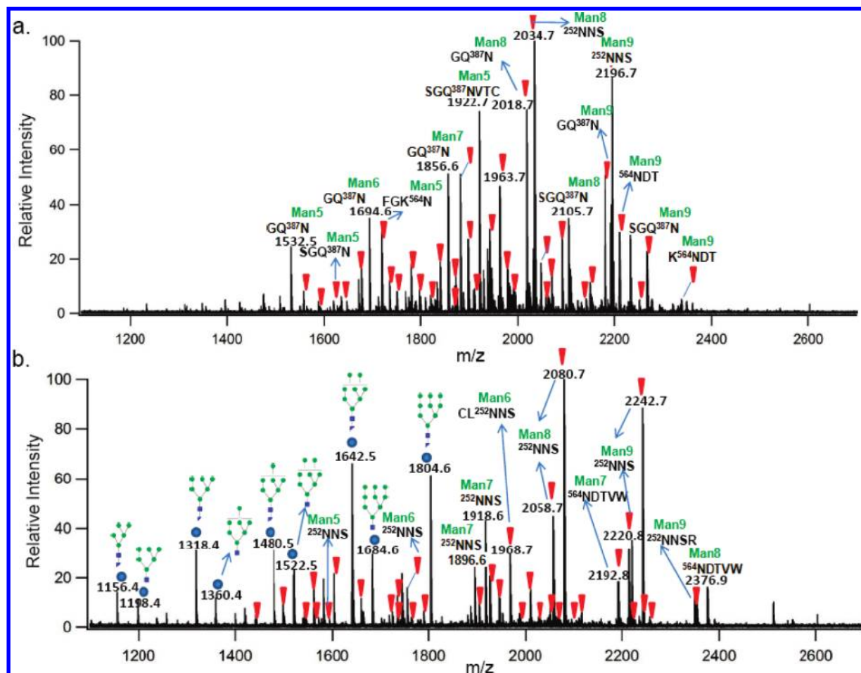
Figure 1. (a) Negative ion mode MALDI FTICR MS spectrum of b-LF glycopeptides after 24 h immobilized pronase digestion. (b) Positive ion mode MS spectrum of the same b-LF glycopeptide sample. Inverted triangles (red ▼) represent potential glycopeptide peaks labeled based on the GP finder analysis of the spectrum mass list, and circles (blue ●) indicate dissociated glycan peaks.
