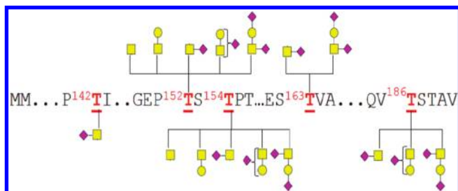
Figure 7. Glycosylation associated with each glycosite of kappa casein (k-CN). The various glycans at each site indicate glycan microheterogeneity in the occupancy of the five glycosites observed during the negative ion mode MS analysis of the k-CN glycopeptides. Rectangles (yellow rectangle), circles (yellow ○), and diamond symbols (pink ◆) represent GalNAc, Gal, and NeuAc residues, respectively.
