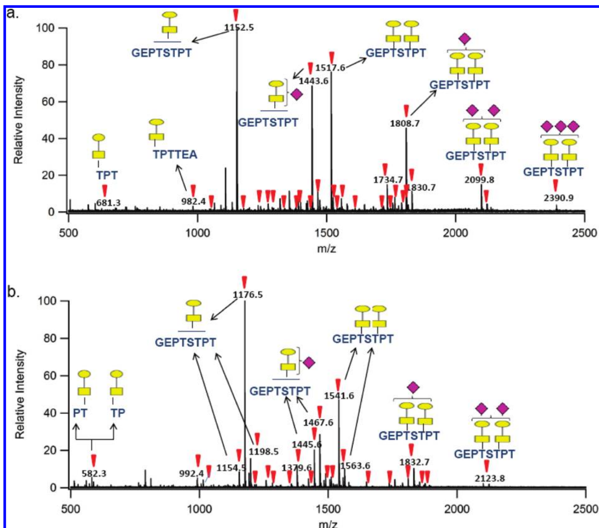
Figure 4. (a) Negative ion mode MALDI FTICR MS spectrum of k-CN glycopeptides after 24 h of reaction with immobilized pronase digestion. (b) Positive ion mode MS spectrum of k-CN glycopeptides from the same sample. Inverted triangles (red \blacktriangledown ) represent potential glycopeptide peaks labeled based on the GP finder analysis of the spectrum mass list. Rectangles (yellow rectangle), circles (yellow \circ ), and diamond symbols (pink \blacklozenge ) represent GalNAc, Gal, and NeuAc residues, respectively.
