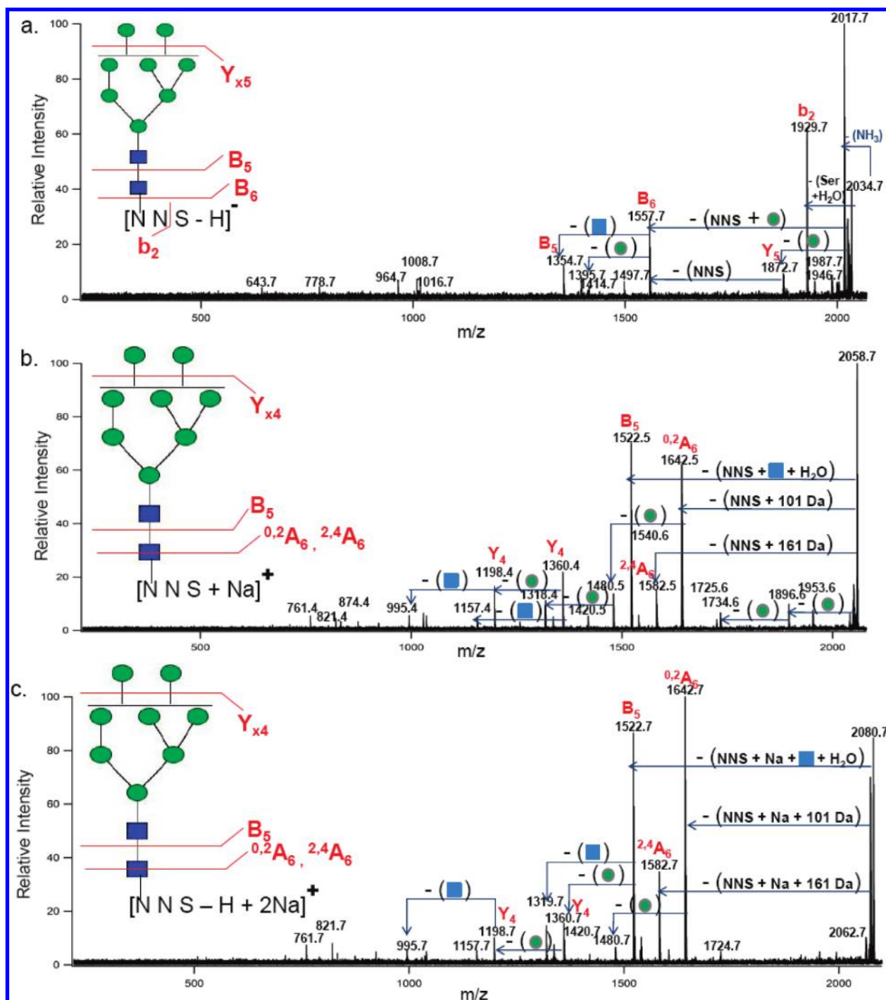
Figure 2. (a) Negative ion mode MALDI FTICR MS/MS spectrum of precursor ion with m/z 2034.70 Da assigned as [^{252}\text{NNS} + \text{GlcNAc}_2 + \text{Man}_8 - \text{H}]^- . (b) Positive ion mode MS/MS spectrum of corresponding sodiated peak with m/z 2058.68 Da assigned as [^{252}\text{NNS} + \text{GlcNAc}_2 + \text{Man}_8 + \text{Na}]^+ . (c) Positive ion mode MS/MS spectrum of a disodiated peak with m/z 2080.68 Da assigned as [^{252}\text{NNS} + \text{GlcNAc}_2 + \text{Man}_8 - \text{H} + 2\text{Na}]^+ . Circles (green ●) and squares (blue ■) represent mannose and GlcNAc residues, respectively.
