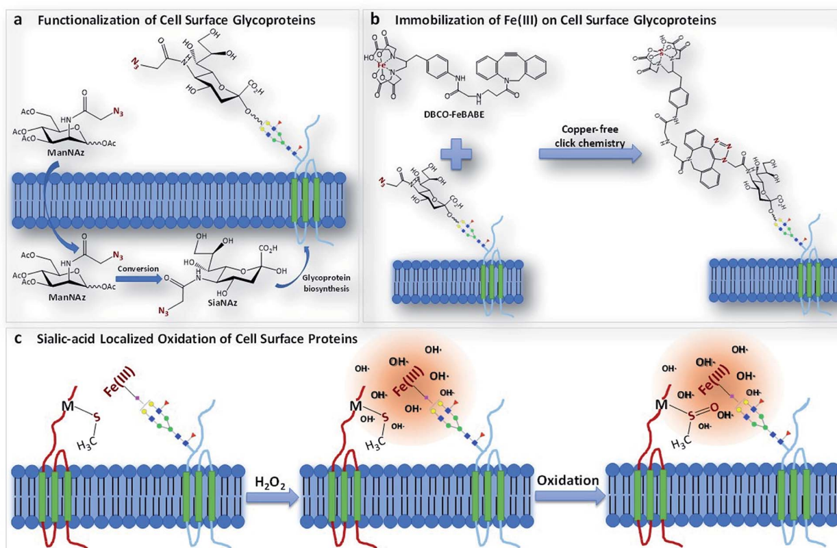
Fig. 1 The schematic representation of the POSE concept. (a) The metabolic incorporation of ManNAz into cell surface glycoproteins as SiaNAz. (b) The bio-orthogonal reaction of the DBCO-FeBABE probe with the SiaNAz group through copper-free click chemistry. (c) The oxidation of proteins in the sialic acid environment by hydroxyl (and other) radicals generated from the reaction between the FeBABE probe and hydrogen peroxide.
